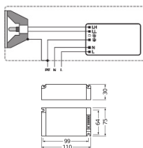
Scheda tecnica Osram LED Driver PowerTronic FIT 35/220 240 S
